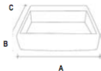
70V01I A = 57.5 cm B = 14 cm C = 46.5 cm
