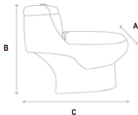
Dubai Plus Blanco - 6MWC5 A = 41 cm B = 65.5 cm C = 73 cm Peso: 43 Kg
