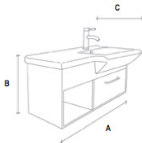
Amazonas 6MBAMA A = 87 cm B = 44 cm C = 47 cm
