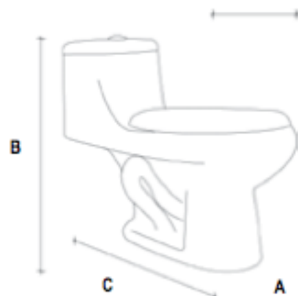
* Dubai Blanco - 6MWC1 A = 39 cm B = 63.5 cm C = 73 cm Peso: 34.30 Kg
