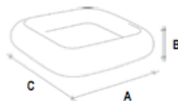
70V06I A = 48 cm B = 11 cm C = 48 cm
