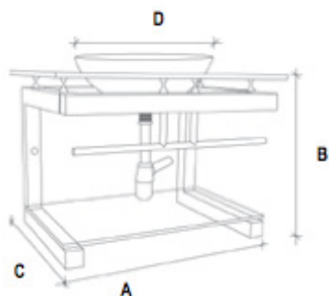
Eufrates 6MBEUFI A = 70 cm B = 50 cm C = 50 cm D = 40 cm
